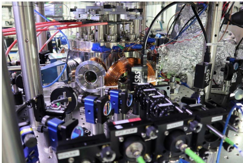
Experimental setup for the cold-atom (neutral-atom) quantum computer at Kenji Ohmori group. (Photograph by Takafumi Tomita)
